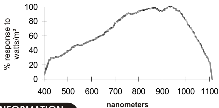
PYRANOMETER SKS 1110
